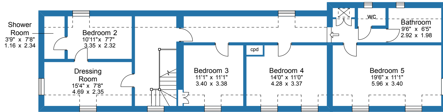
First Floor
